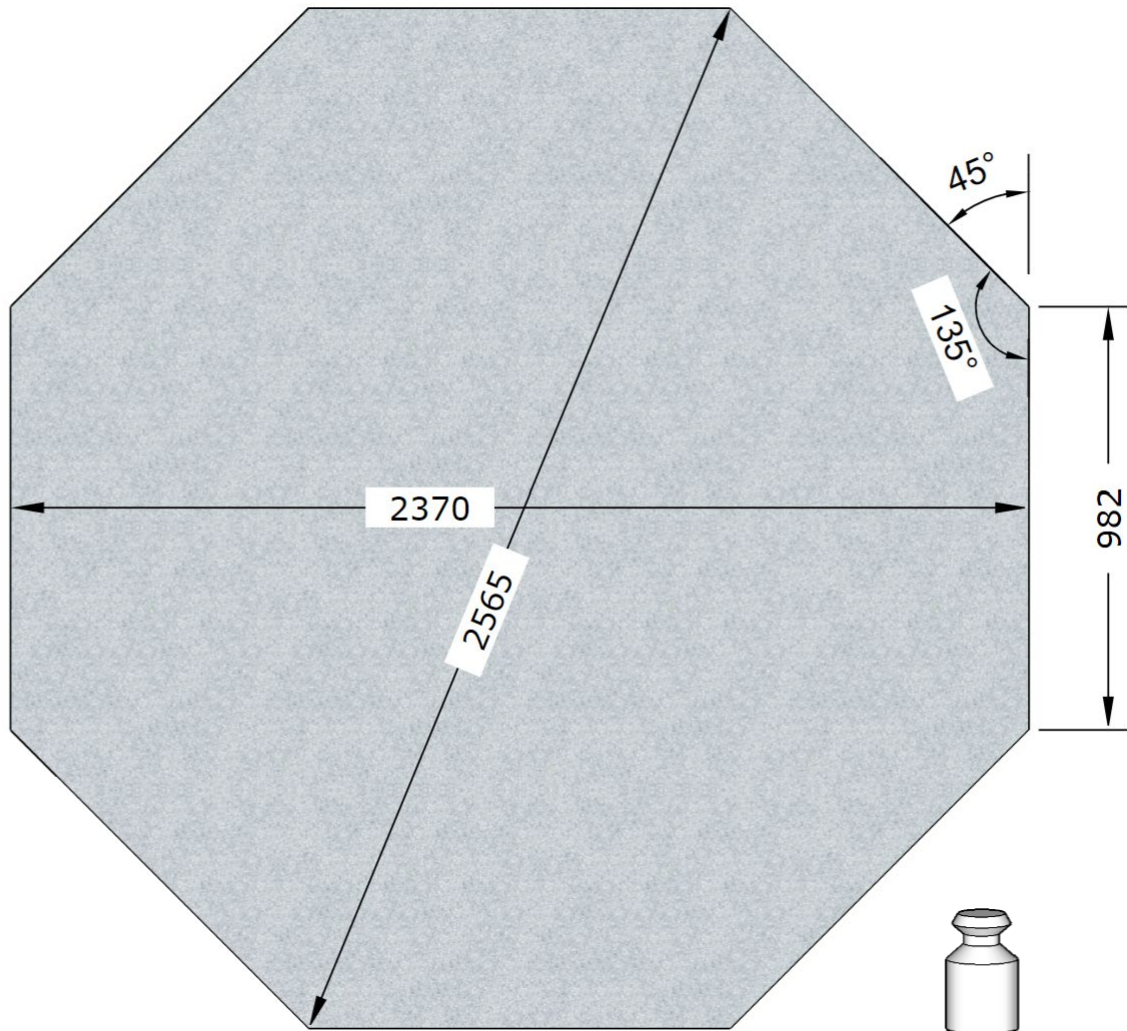
Concrete Foundation
